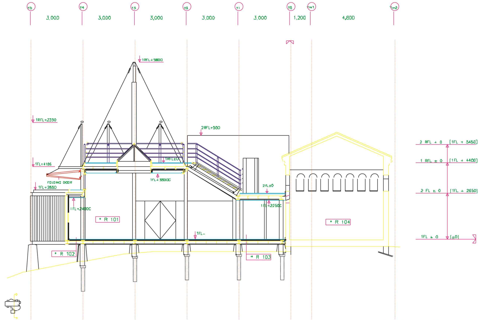
SECTION AA'
