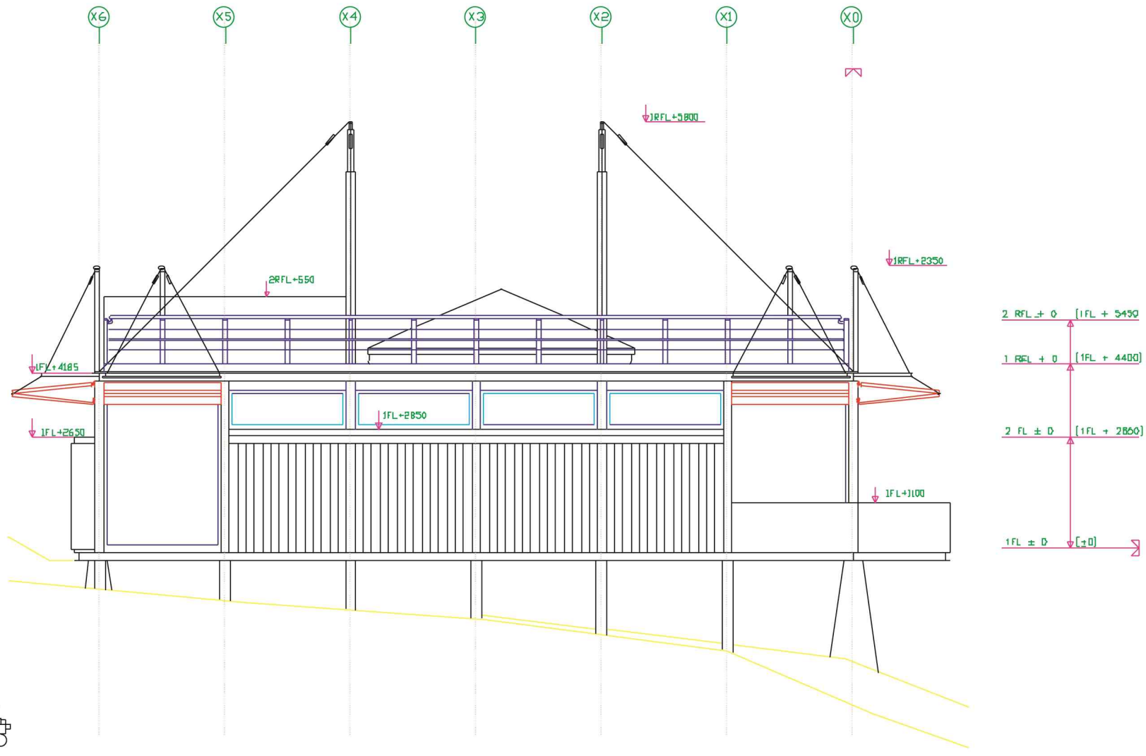
ELEVATION NORTH
