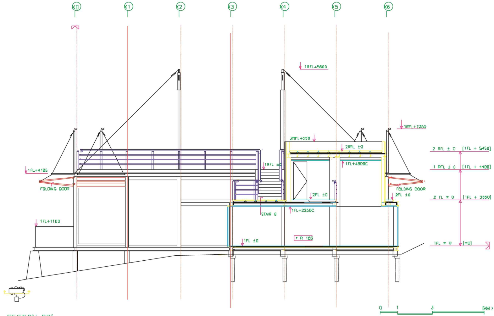
SECTION DD'
